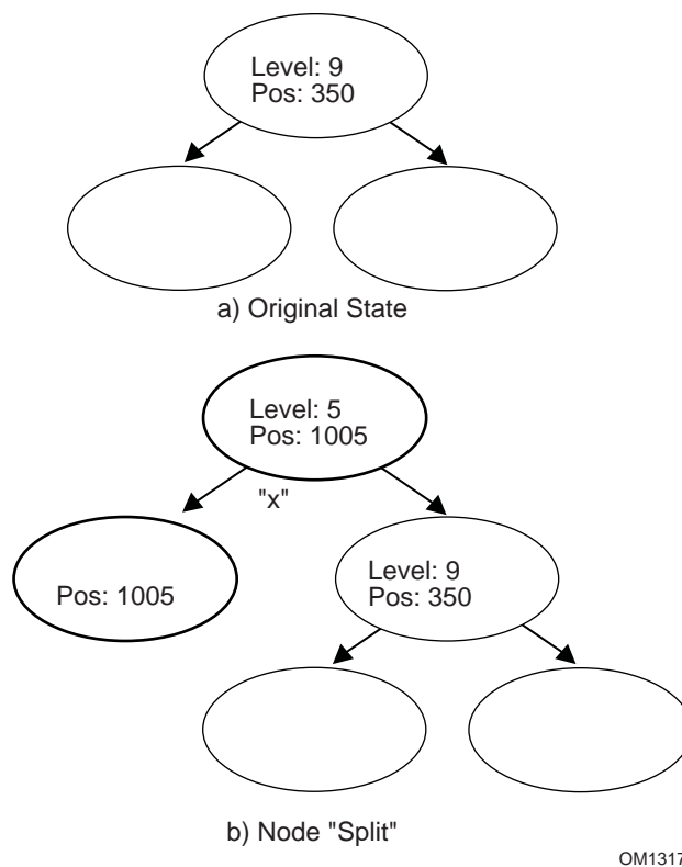
Figure 68. Node Split
