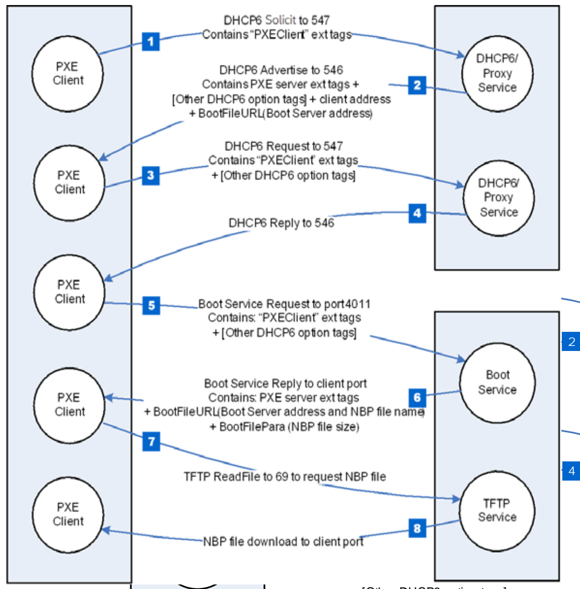
Figure 75. IPv6-based PXE boot
