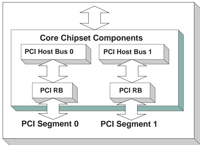
Figure 43. Server System with Two PCI Host Buses
