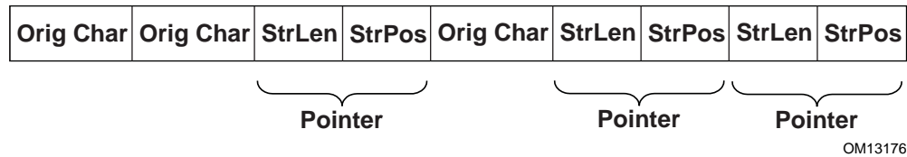
Figure 66. Block Body
