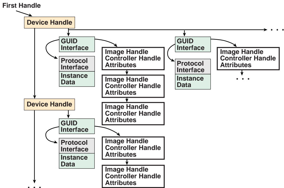
Figure 26. Handle Database
