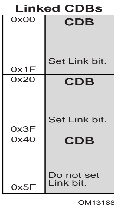
Figure 157. Linked CDBs
